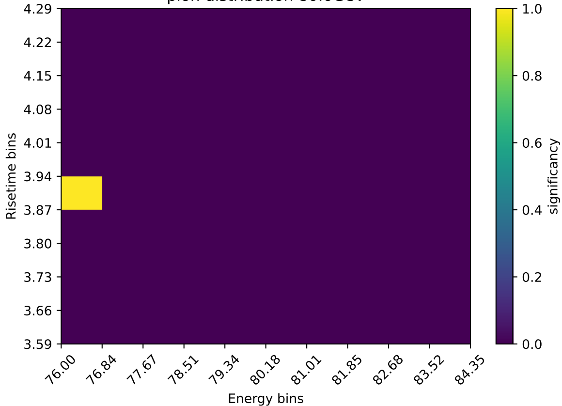
pion distribution 80.0GeV
